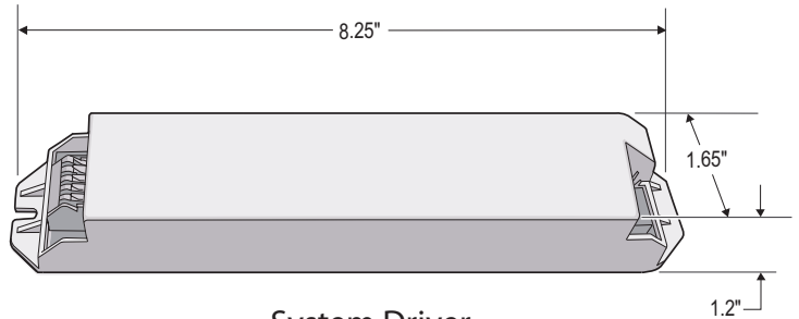
- System Driver -
