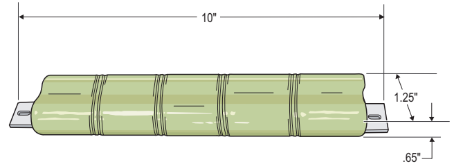
- 30 Minute Battery -
